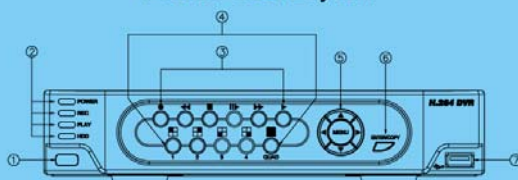
Front Panel Layout
